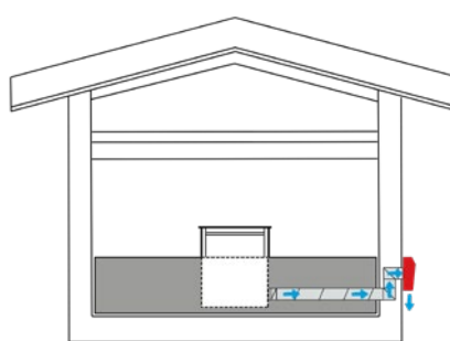
SEM21/71 Motor - duct from the units side, through the cabinet, out the wall, to the external wall motor
